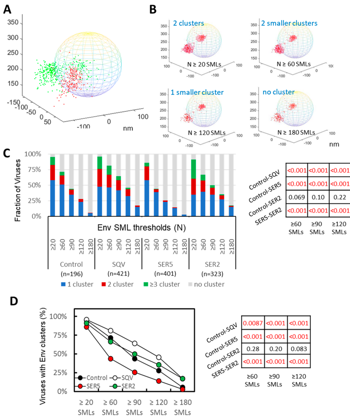
Figure 4. 3D iPALM imaging and analysis of HIV-1 Env distribution on virions. (A) Illustration of 2-color 3D iPALM imaging on single Env molecule localizations (SMLs, red dots) and SER5 SMLs (green dots) projected onto a 200 nm diameter sphere representing a GFP-Vpr labeled viral particle. (B) Illustration of Env SMLs (red dots) in 3D overlaid onto an idealized viral particle shown as a sphere with diameter of 200 nm. Dependence of Env clustering (light red area) on the DBSCAN SML threshold N of 20, 60, 120, and 180 localizations and the same searching distance R of 20 nm. X , Y , Z axes are in nm. (C) Analysis of Env clustering for a panel of HIV-1 pseudoviruses consisting of control and immature (SQV) particles and virions containing SER2 and SER5, using different DBSCAN SML threshold parameters, as indicated. The results are categorized into no cluster, 1, 2, and \geq 3 clusters per virion. The same R = 20 nm for DBSCAN analysis with N = 20, 60, 90, 120, and 180 localizations. (D) Fraction of pseudoviruses containing or lacking Env clusters (two categories) for the same DBSCAN parameters as in B. Statistical analyses of data in panel B and C using Fisher's Exact Test are shown on the right.
