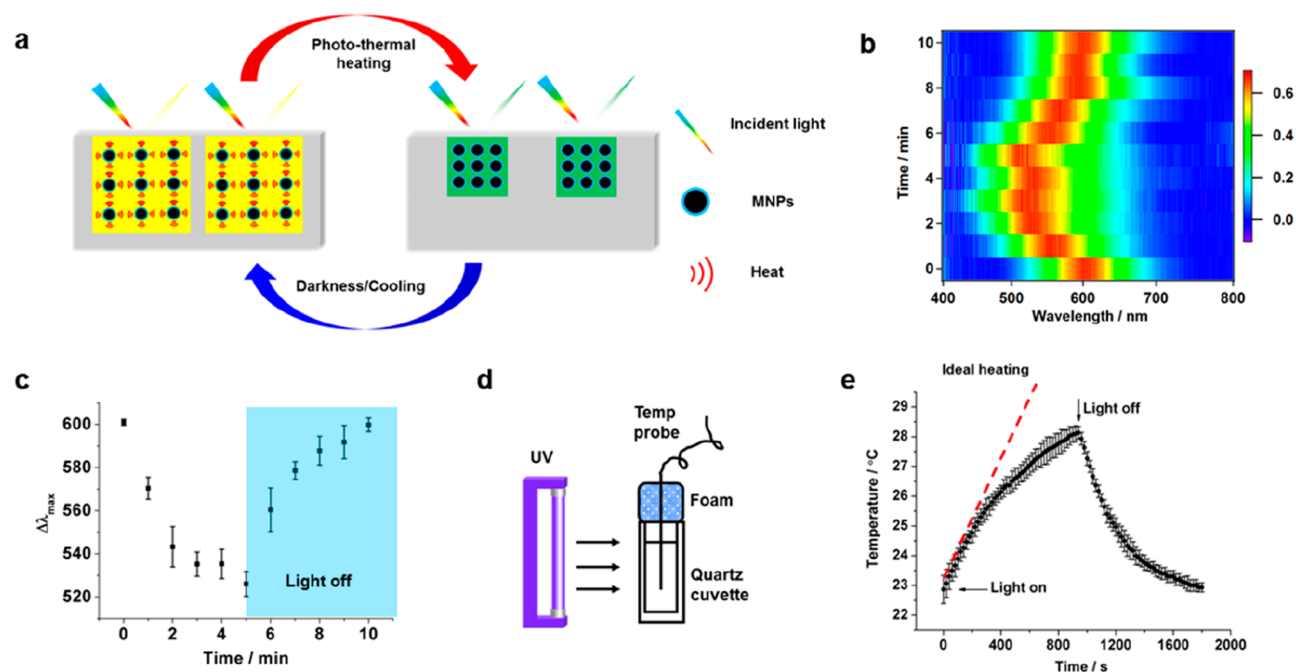
Figure 3. Light-responsive behavior of SASS. (a) Schematic of the light-responsive mechanism of SASS. Exposure to white light induces photothermal heating and a concomitant spectral shift in the peak absorbance as the spacing within the PC decreases. Cessation of light returns SASS to its original state. (b) Two-dimensional color map depicting the spectral shift of SASS as a function of time when exposed to a white light LED source (light was on 0–5 min and off 5–10 min). (c) Reflection \lambda_{\text{max}} of illuminated SASS samples as described in (b). The error bars represent the standard deviation of three measurements obtained from three different SASS samples. (d) Schematic of equipment setup used for measuring the photothermal conversion efficiency. A UV light source was used to illuminate a dispersion of MNPs while the solution temperature was measured. (e) Plot of solution temperature during exposure of MNP dispersion to UV light as a function of time. The error bars represent the standard deviation from three independent samples. The red dashed line indicates the ideal heating of the dispersion and provides the heating rate of the sample.
