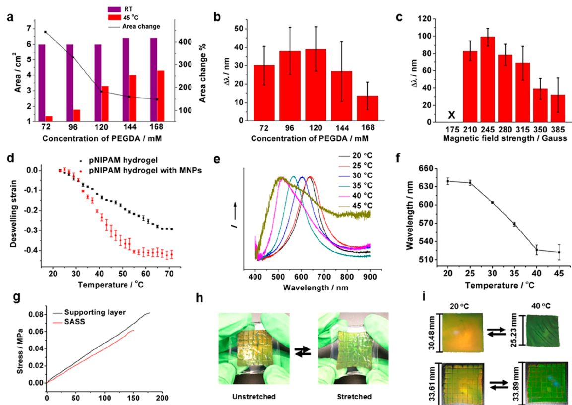
Figure 2. Characterization of SASS. (a) Plot relating the cross-linker (PEGDA) concentration in pNIPAM PC gels to their area before and after heating to 45 °C (a 350 G magnetic field was applied during polymerization). The right y-axis represents the area change % upon heating for each composition. (b) Plot showing the change in reflection \lambda_{\max} for the samples prepared in (a). The \Delta\lambda_{\max} was determined using reflection spectra of standalone PC films at RT and 45 °C. (c) Plot of reflection \Delta\lambda_{\max} (collected at RT and 45 °C) for responsive pNIPAM PCs polymerized under different magnetic field strengths. These gels were synthesized with 120 mM PEGDA. (d) Plot of temperature-dependent strain of pNIPAM hydrogels prepared without (black) and with magnetic nanoparticles (red). (e) Normalized reflection spectra of a SASS sample collected at different temperatures. (f) Plot showing \lambda_{\max} of reflectance for SASS samples as a function of temperature. (g) Representative uniaxial tensile measurement of a SASS sample (red) and a sample of a standalone film comprised of the strain-accommodating polymer (black). (h) Photographs demonstrating the elasticity of SASS and its strain-induced color change. (i) Photographs showing the chromatic response of a traditional responsive pNIPAM PC film (upper) triggered by adjusting the temperature (20 to 40 °C) compared to the chromatic response of SASS (lower) under the same conditions. The dimensions of the materials in the initial and final states are provided to the left of each image. All error bars represent the standard deviation of three independent measurements.
