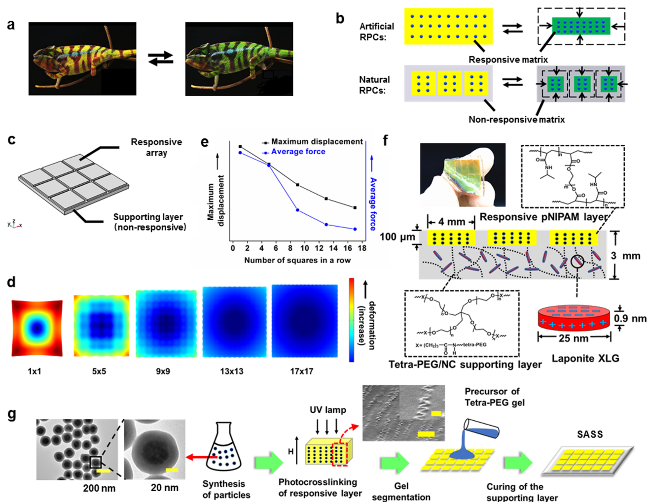
Figure 1. Design and fabrication of strain-accommodating smart skin (SASS) material. (a) Photographs of a chameleon displaying color change (adapted with permission from Teyssier, J., Saenko, S. V., van der Marel, D., and Milinkovitch, M. C. Nat. Commun. 2015, 6, 6368; copyright 2015 Springer Nature). 1 (b) Schematic comparing the typical design of artificial responsive PCs to responsive PCs utilized by nature. The dots represent the PC, yellow and green represent the swollen and deswollen states of the responsive hydrogel, respectively, and gray indicates the supporting, nonresponsive polymer matrix. (c) Model used for finite element analysis (FEA) of SASS (also see Figure S1). (d) Rendering of FEA model mapping the deformation of a bilayer material with a supporting nonresponsive layer and a responsive upper layer divided into sections. (e) Plot of the FEA-determined average force and maximal displacement within a plane of the supporting polymer layer as a function of the number of squares in the responsive PC array layer. (f) Photograph and schematic of SASS that includes dimensions and chemical structure of polymers. (g) Flow diagram illustrating the steps used in SASS fabrication, where TEM and SEM images show representative structures of the magnetic nanoparticles and their organization with the responsive PC (scale bar of SEM image: 5 and 1 \mu\text{m} (inset)).
